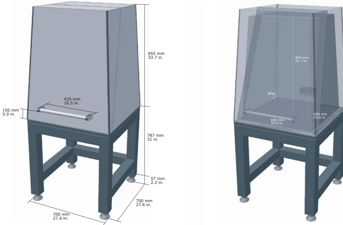
▲ Fig. 1: Dimensions of Acoustic Enclosure 600 mounted to optional steel frame, which needs to be ordered separately!
