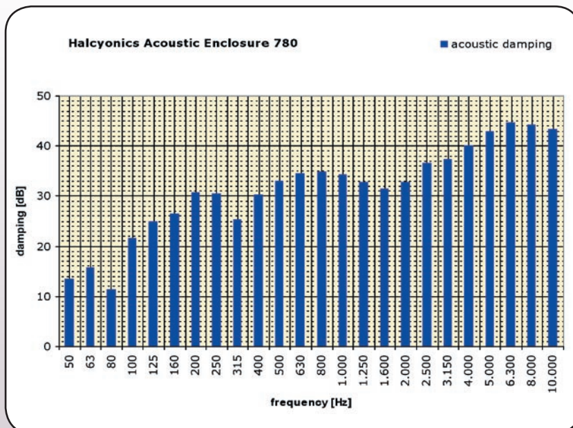
▲ Fig. 2: The above measurement has been performed with an Acoustic Enclosure 780. The damping performance of the Acoustic Enclosure 600 is comparable or even better.
